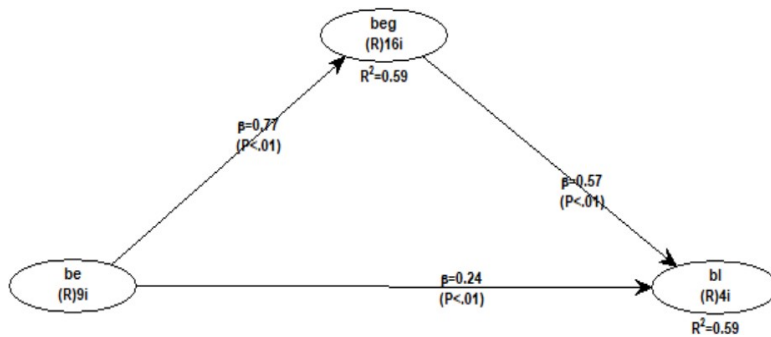
Figure 2. Structural Equation
